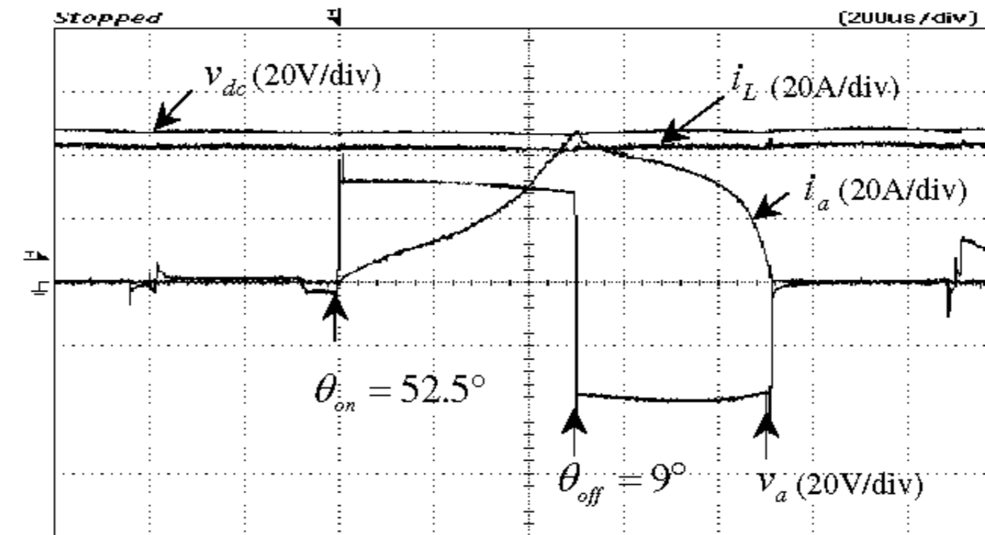
Figure 28. Measured results of phase voltage v_a , phase current i_a , dc-link voltage v_{dc} and load current i_L at 6000 rpm, \theta_{on} = 52.5^\circ , \theta_{off} = 9^\circ , R_L = 1.2\Omega
