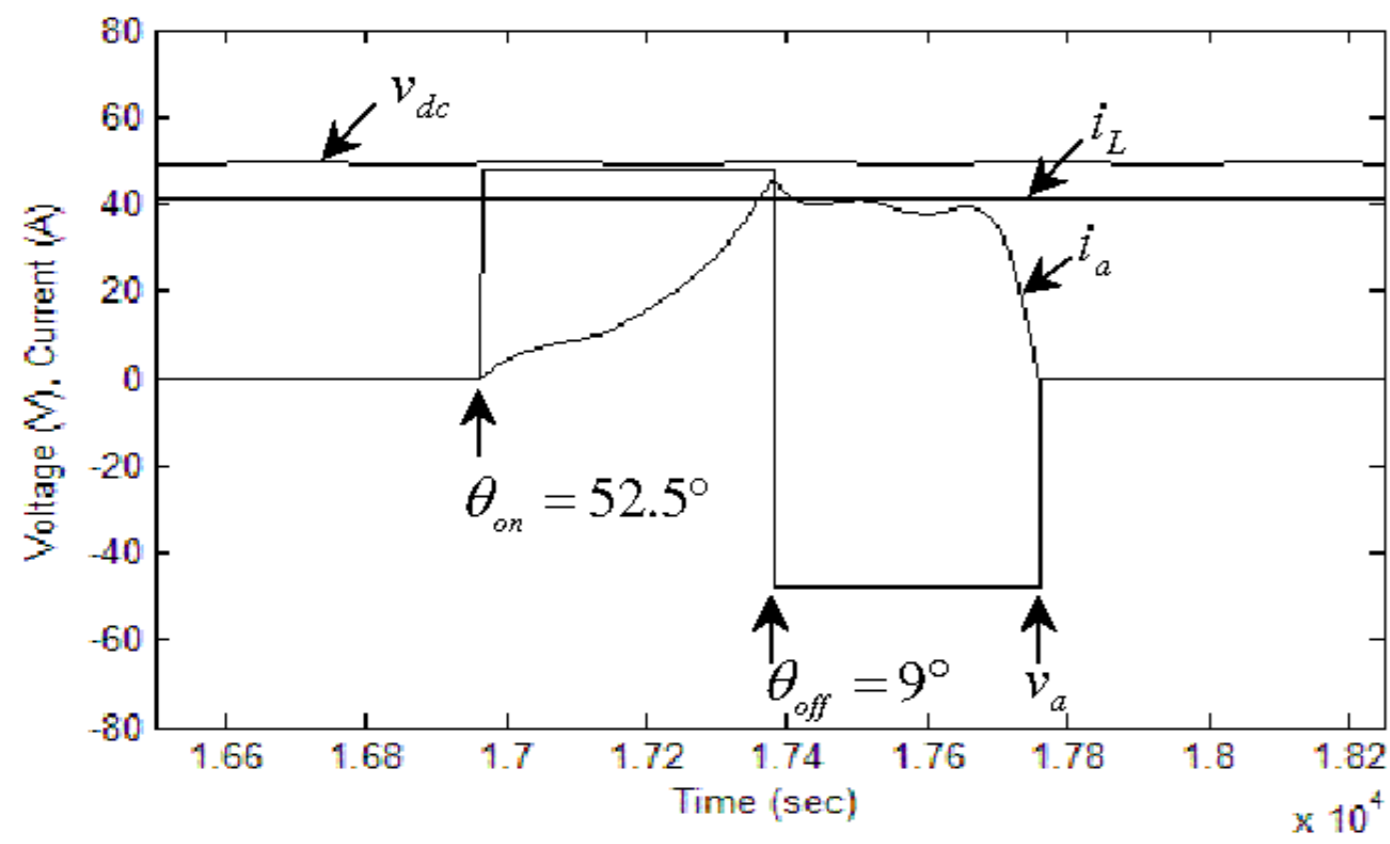
Figure 23. Simulation results of phase voltage v_a , phase current i_a , dc-link voltage v_{dc} , and load current i_L at 7000 rpm, \theta_{on} = 52.5^\circ , \theta_{off} = 9^\circ , R_L = 1.2\Omega
