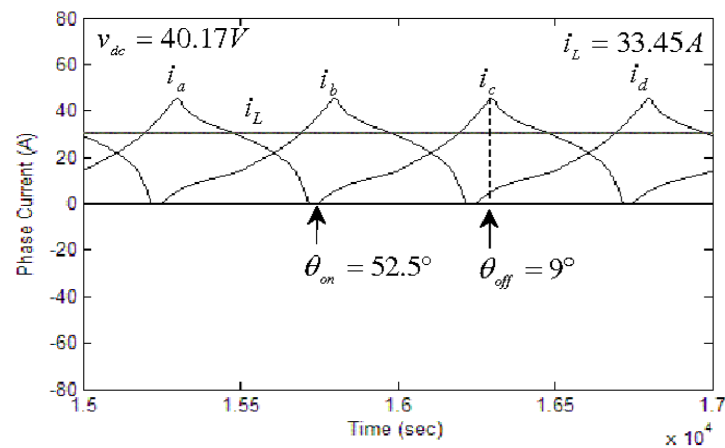
Figure 25. Simulation results of phase currents i_a, i_b, i_c, i_d and load current i_L at 5000 rpm, \theta_{on} = 52.5^\circ , \theta_{off} = 9^\circ , R_L = 1.2\Omega
