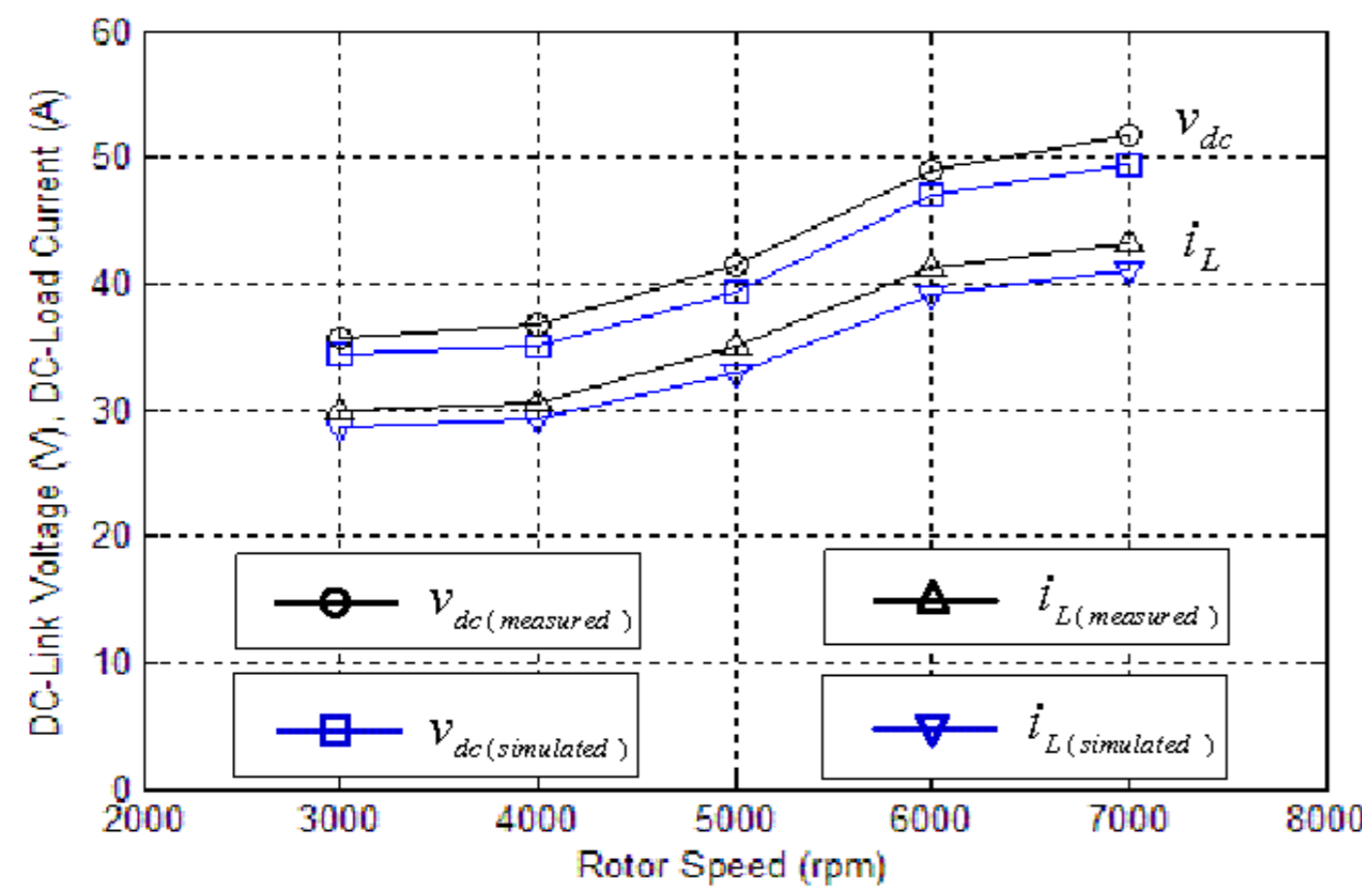
Figure 26. The relationship of the simulated and measured results of the dc-link voltage v_{dc} and the dc-load current i_L versus rotor speed \omega , at \theta_{on} = 52.5^\circ and \theta_{off} = 9^\circ and R_L = 1.2\Omega
