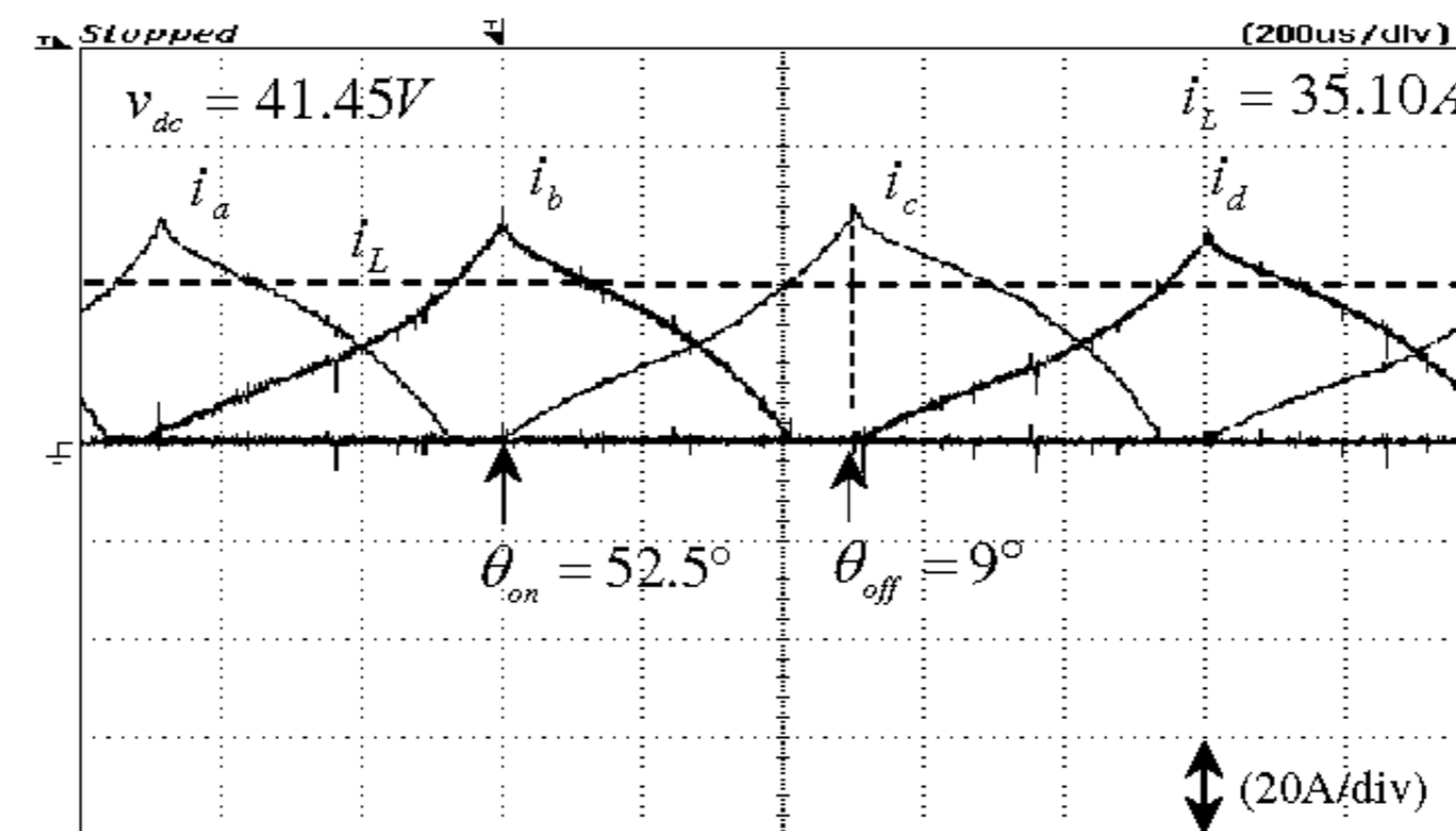
Figure 29. Measured results of phase currents i_a, i_b, i_c, i_d and load current i_L at 5000 rpm, \theta_{on} = 52.5^\circ , \theta_{off} = 9^\circ , R_L = 1.2\Omega
