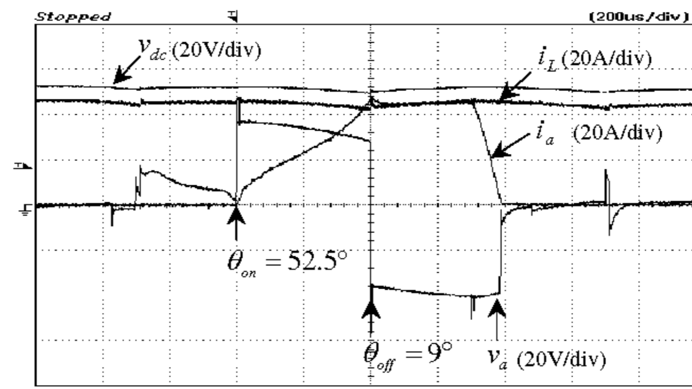
Figure 27. Measured results of phase voltage v_a , phase current i_a , dc-link voltage v_{dc} and load current i_L at 7000 rpm, \theta_{on} = 52.5^\circ , \theta_{off} = 9^\circ , R_L = 1.2\Omega
