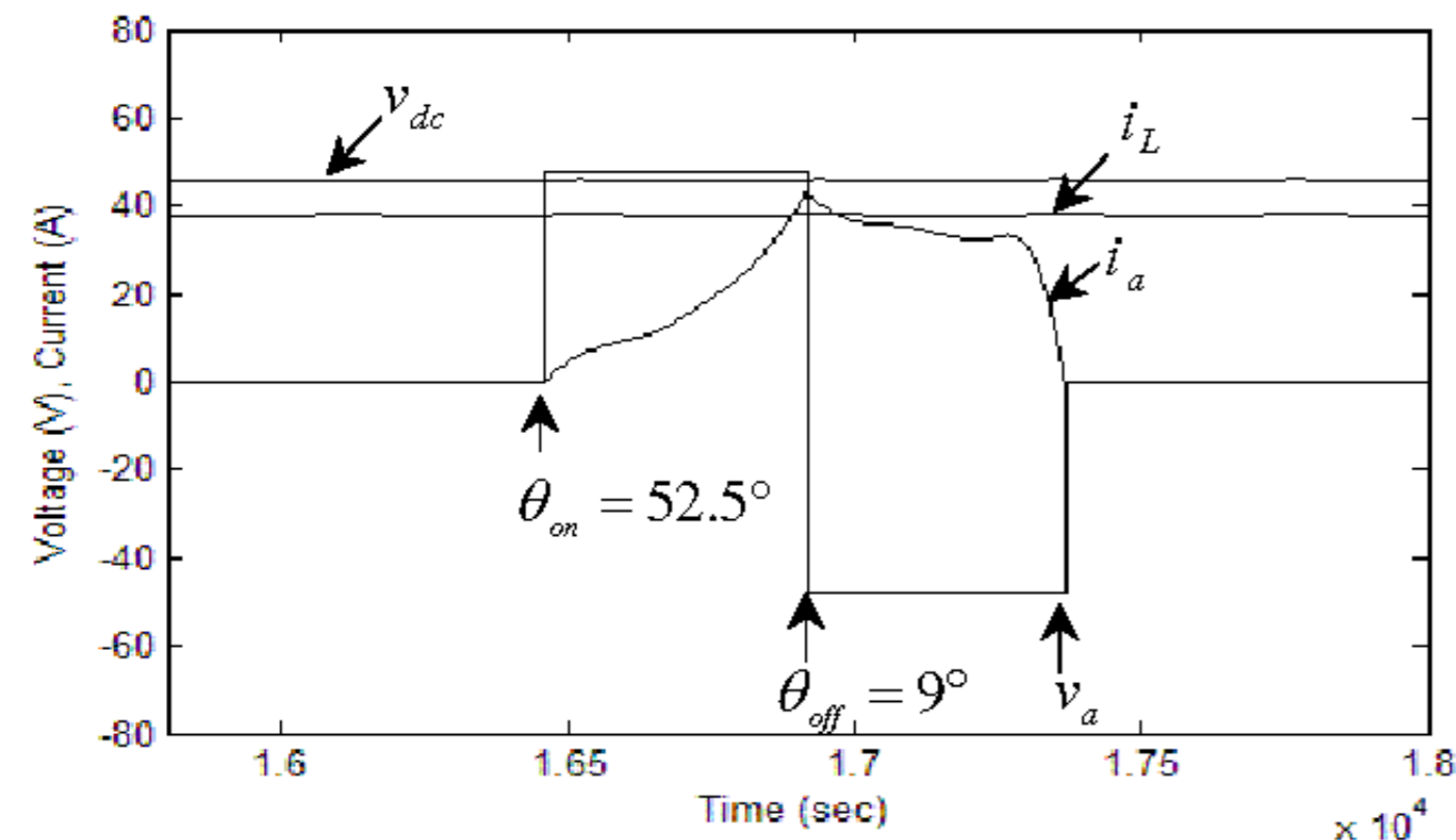
Figure 24. Simulation results of phase voltage v_a , phase current i_a , dc-link voltage v_{dc} and load current i_L at 6000 rpm, \theta_{on} = 52.5^\circ , \theta_{off} = 9^\circ , R_L = 1.2\Omega
