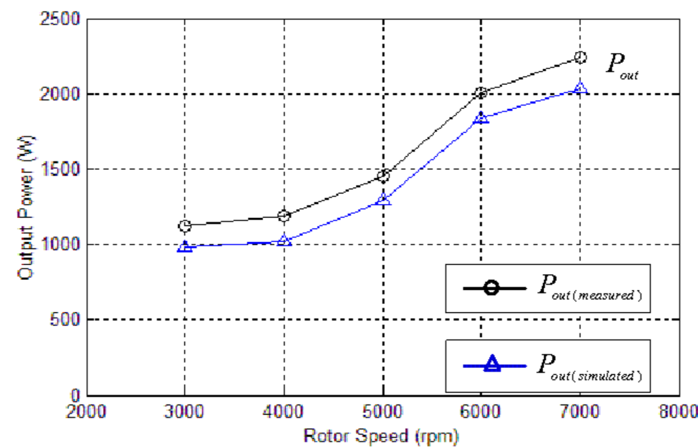
Figure 30. The relationship of the simulated and measured output power P_{out} versus rotor speed \omega , at \theta_{on} = 52.5^\circ and \theta_{off} = 9^\circ and R_L = 1.2\Omega
